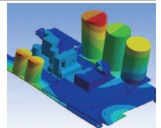
3D-vibration analysis
